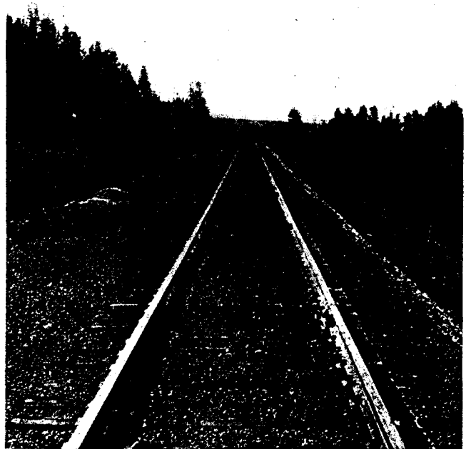
Slag ballasted track on the Denver & Rio Grande Western main line between Tennessee Pass, Colo., and Keeldar
