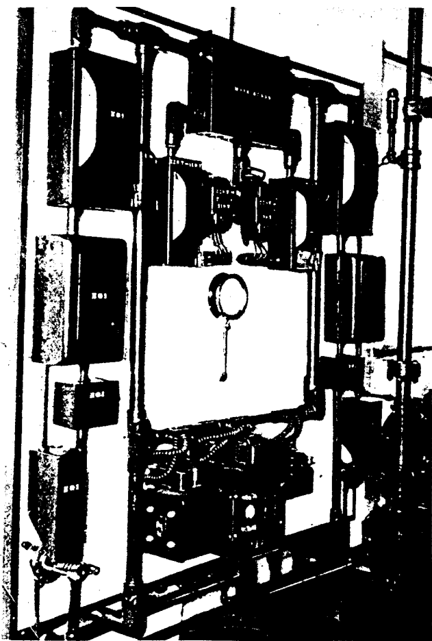
Power board at "KC," showing transformers, air gages and control equipment mounted on asbestos panel
